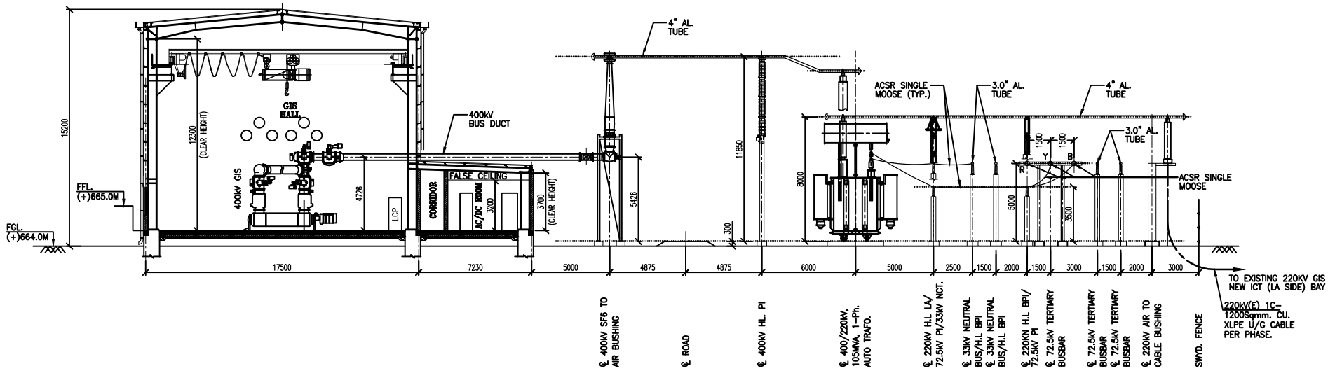
SECTION : B-B (400kV TRAF. BAY, 220kV LINE BAY AND 72.5kV TERTIARY BAY) (SCALE-1:250)
